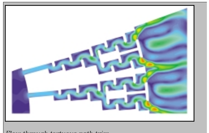
Flow through tortuous path trim.
