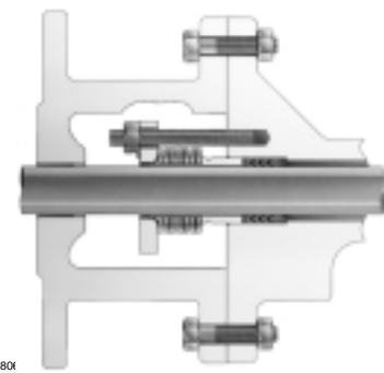
ENVIRO-SEAL® Packing System (Single PTFE V-Ring)
